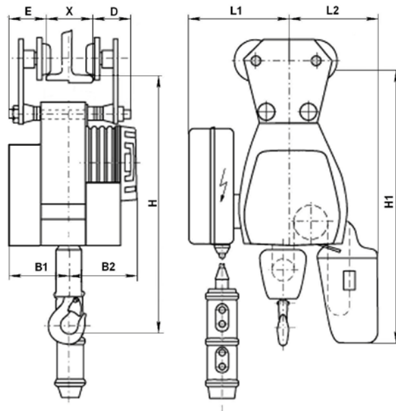
push trolley
