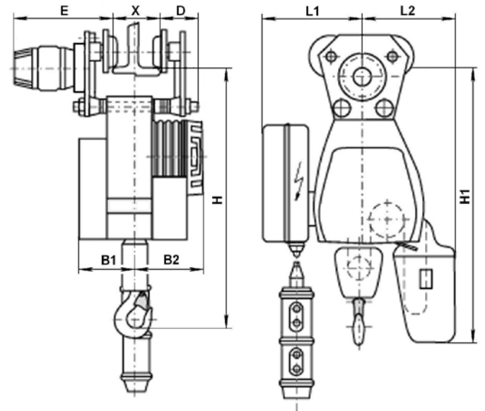
motorized trolley
